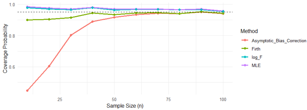
Figure 16: Estimated coverage probability of 95% Wald CI for \beta_1 in extreme case ( \beta_0 = -3, \beta_1 = 1, m_1 = 1 ).
