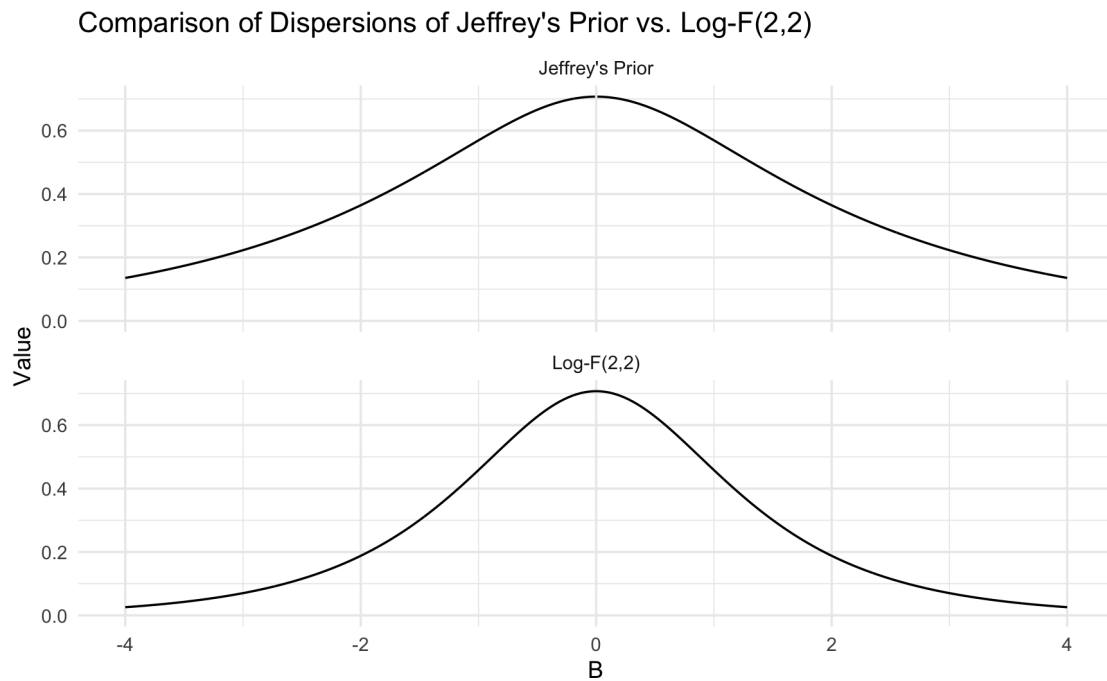
Figure 4: Jeffrey's Prior vs log-F(2, 2)
