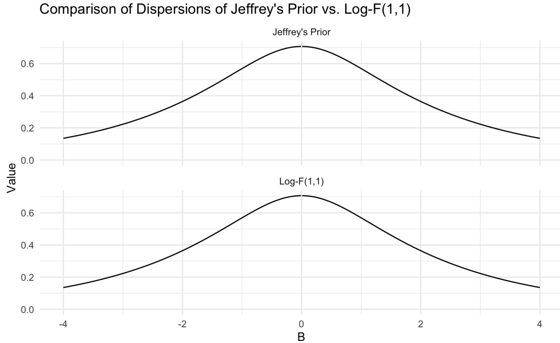
Figure 3: Jeffrey's Prior vs log-F(1,1)
