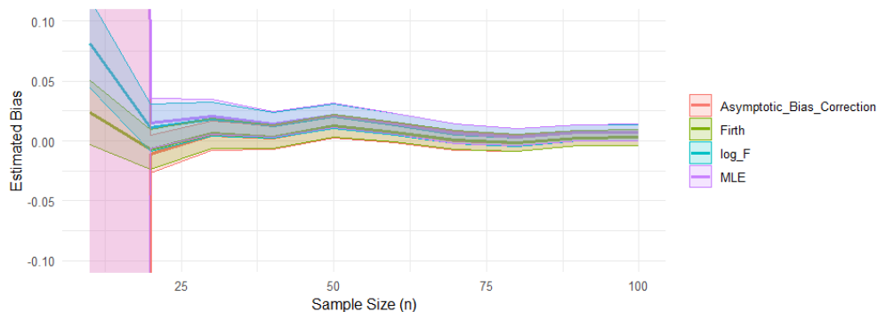
Figure 9: Estimated bias of \hat{\beta}_1 with 95% confidence intervals in easy case ( \beta_0 = 0, \beta_1 = 0.1, m_1 = 1 ).
